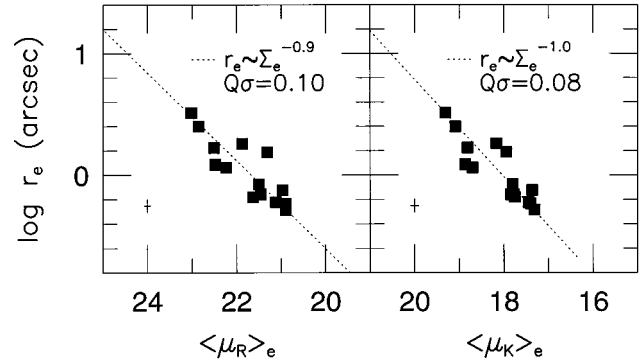
FIG. 1.—Comparison of the Kormendy relations in the R_C band (left) and K band (right) for cluster Abell 851 at z = 0.407 . The data are well fit by the Kormendy relation slopes, as shown in the figure, with quartile-estimated rms residuals in \log r_e from each relation given as Q\sigma .
