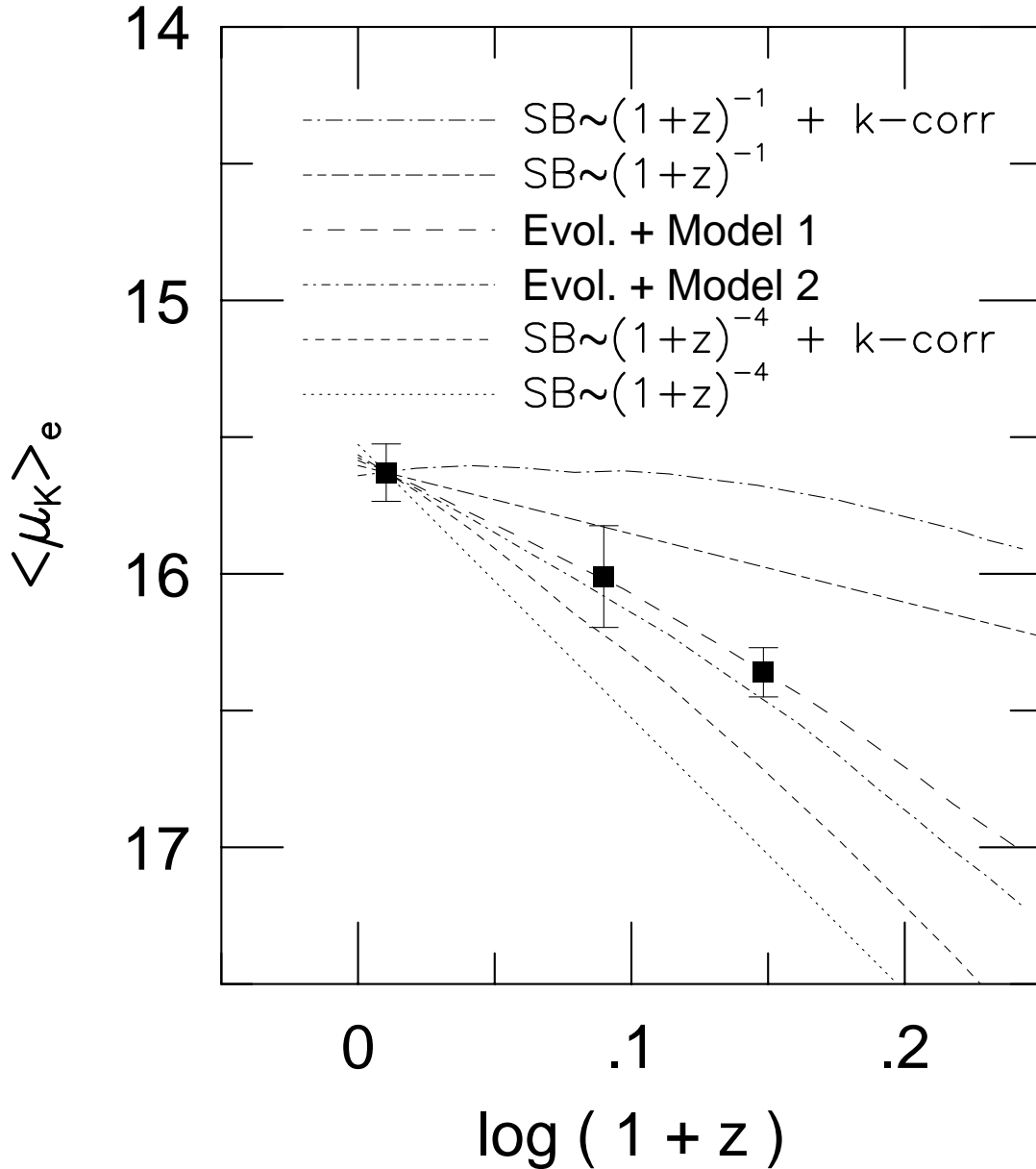
Fig. 2.— The Tolman SB test in the K -band using the intercepts on the \langle \mu \rangle_e axis where R_e = 1 kpc ( H_0 = 75 km s ^{-1} Mpc ^{-1} , \Omega_0 = 0.2 , and \Lambda_0 = 0 ). The data are uncorrected for SB dimming, nor has a k -correction been applied. Plotted for comparison are the expansion (1+z)^{-4} and non-expansion (1+z)^{-1} models, both with and without a k -correction. Models 1 and 2 (from Buzzoni 1995) both include SB dimming, a k -correction, and passive evolution (Evol.) using cosmological parameters ( H_0, \Omega_0, z_f ) of (50, 0.5, \infty ) and (100, 0, \infty ), respectively. The data are consistent with luminosity evolution in the cluster elliptical galaxy population as predicted by the simple stellar population models.
