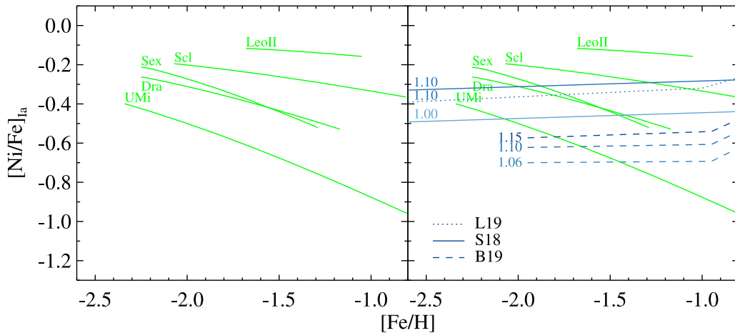
Figure 8. Metallicity dependence of observationally inferred (green) and theoretical (shades of blue) [\text{Ni}/\text{Fe}]_{\text{Ia}} yields for sub- M_{\text{Ch}} SNe Ia. The blue numbers indicate the WD mass in M_{\odot} . Both panels show the same data, but the theoretical predictions are suppressed in the left panel for clarity. The line style for each theoretical prediction reflects the study from which it came, and the shading indicates the initial WD mass, consistent with Figure 6.
