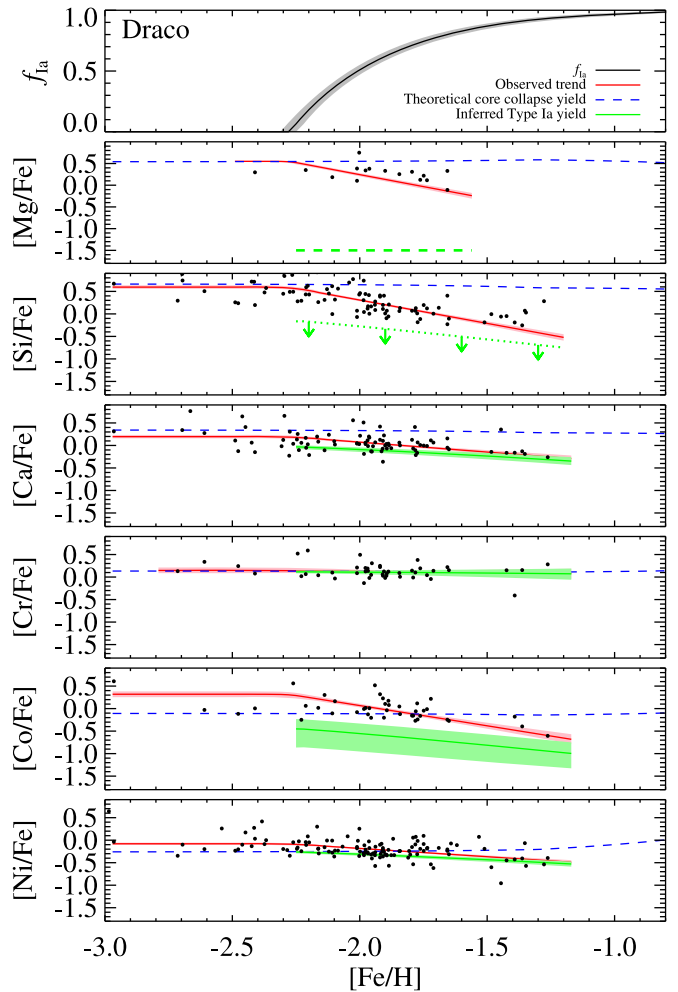
Figure 3. Same as Figure 1 but for Draco.
