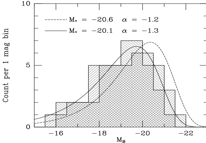
Figure 1. The observed distribution of GRB host galaxy absolute magnitudes in the restframe B band (histograms), fitted by the luminosity-weighted Schechter luminosity function (solid line). The two histograms represent the same data, with the binning offset by half a bin. The dashed line corresponds to the z \sim 0 GLF for all morphological types, from the 2df redshift survey.
