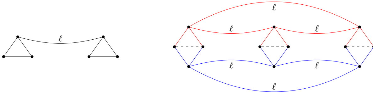
Figure 2: H , draw on the left, consists of two triangles joined by a path of length \ell . On the right, F_{red} is drawn in red, F_{blue} in blue and the matching M is drawn with dashed lines.
