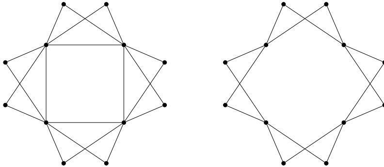
Figure 1: C_4 \ominus_2 K_3 (on the left) and C_4 \odot_2 K_3 (on the right).
