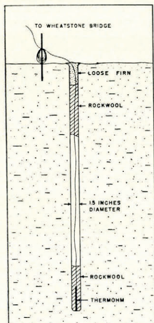
Fig. 4. Thermohm as installed in firn in 1949
