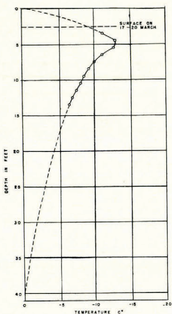
Fig. 6. Quasi-hypothetical curve for chilled layer of 1949-50 based on temperature measurements of 18-20 March 1950, by Walter A. Wood
