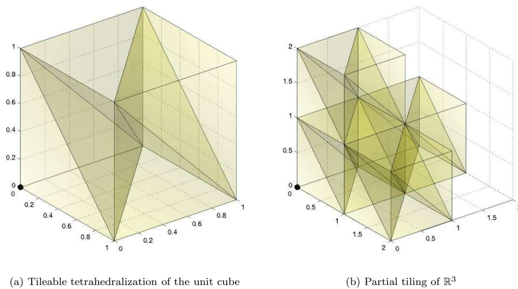
FIGURE 18. Regular tiling of \mathbb{R}^3 that admits a generalized cone operator.
