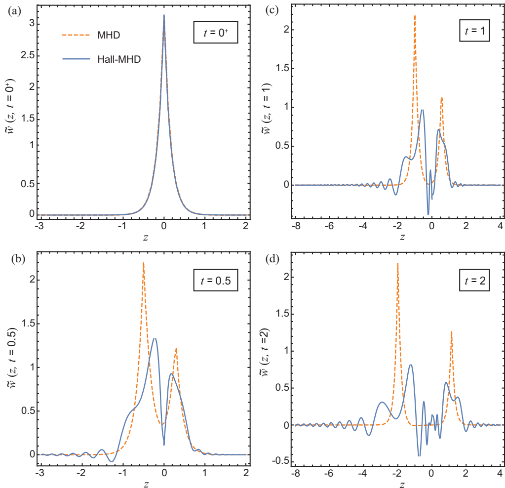
FIG. 5. Normal velocity profile from the IICE model, \tilde{w}(z, t) , for t = 0^+ , 0.5, 1, 2, in (a)–(d), respectively. The Hall-MHD solutions, obtained for \beta = 2 , d_L = d_S = 0.1 , and \mathcal{A} = 0.5 , given by the solid lines, are compared to the regular MHD solutions of the same energy ratio and Atwood number, shown as dashed lines.
