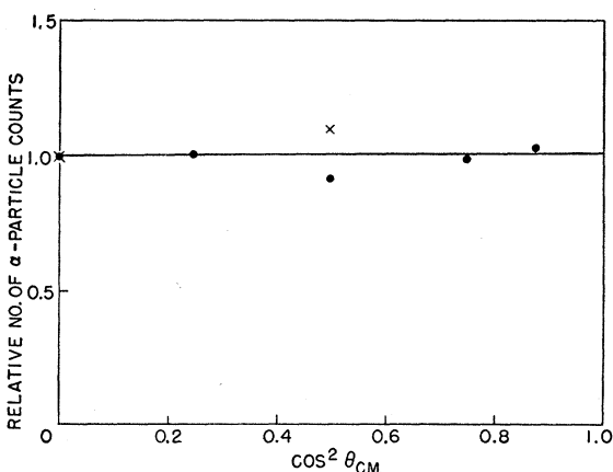
FIG. 10. Angular distribution of the \alpha_3 group from the F^{19}(p,\alpha)O^{16*} reaction at a bombarding energy of 1381 keV; the crosses are points taken at angles forward of 90^\circ and the circles are back angle points; the solid curve is W(\theta) = 1 .
