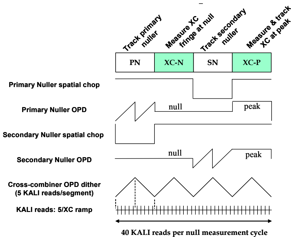
Figure 2. Nuller micro-sequence.
