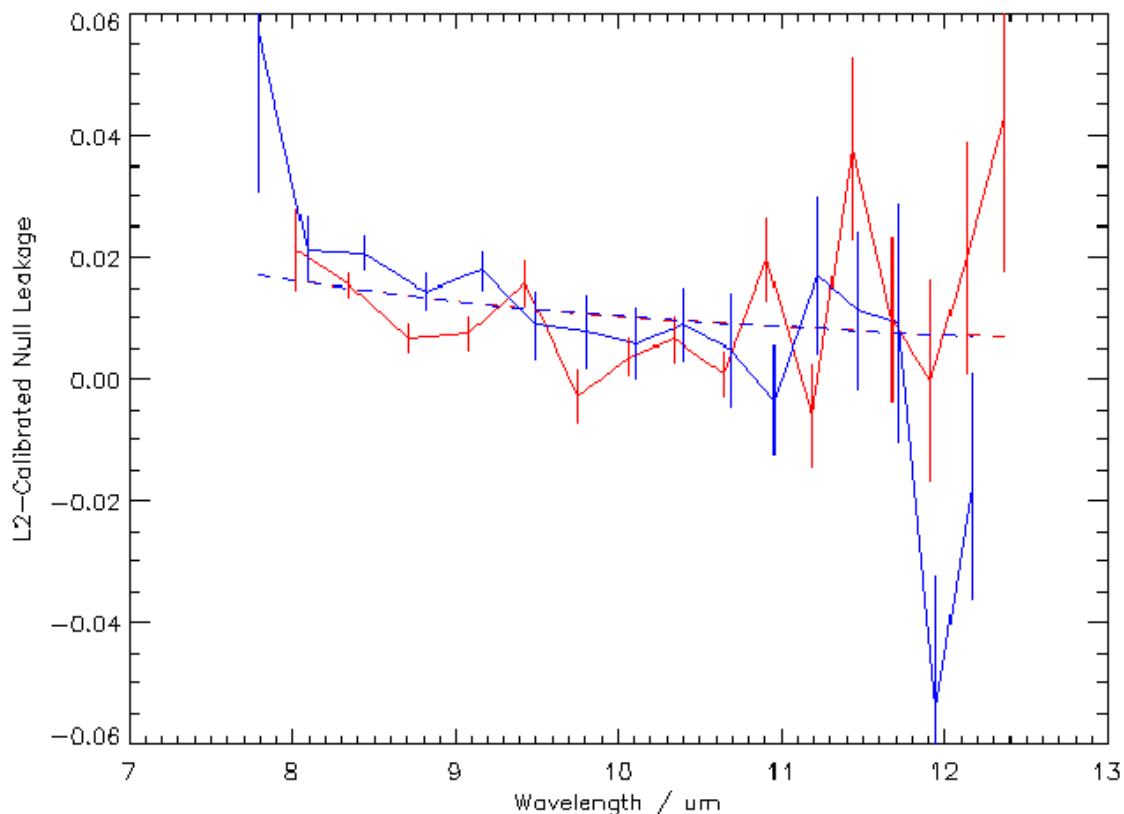
Figure 4. Preliminary calibrated null depth vs. wavelength from April 2006. The solid curves are null leakage vs. wavelength on the two nuller ports, and the dotted curve is the theoretical prediction.
