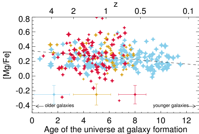
Figure 6. The dependence of [\text{Mg}/\text{Fe}] on formation redshift. The median uncertainties are shown in the bottom. The color scheme follows previous plots (indicating different observed redshifts). A slight negative slope suggests that quiescent galaxies that form earlier on average had shorter star formation duration.
