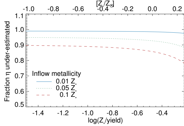
Figure 11. The underestimation of the mass-loading factor (the ratio between \eta derived assuming pristine inflowing gas to \eta derived with enriched inflow) as a function of stellar metallicity. The bottom x -axis is the metallicity in units of the yield. The top x -axis shows the metallicity when the yield is assumed to be 3Z_{\odot} . Each line corresponds to a different assumed metallicity of the inflow.
