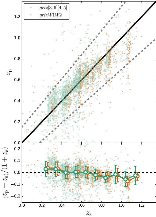
Figure 3. The plot of photo- z versus spec- z (top) and of photo- z mean error and RMS scatter (bottom) for the galaxy sample. Photo- z 's are measured using SED fitting with either griz [3.6][4.5] (red) or griz W1W2 (green) photometry. The dashed lines in the upper panel bracket the region with \|\Delta z\|/(1+z) < 0.15 . For clarity, these two samples are plotted with an offset of 0.02 on the x -axis.
